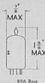
B9A Base
